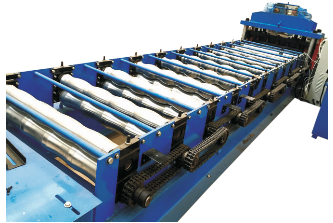
SINGLE LAYER ROLL FORMING MACHINE
