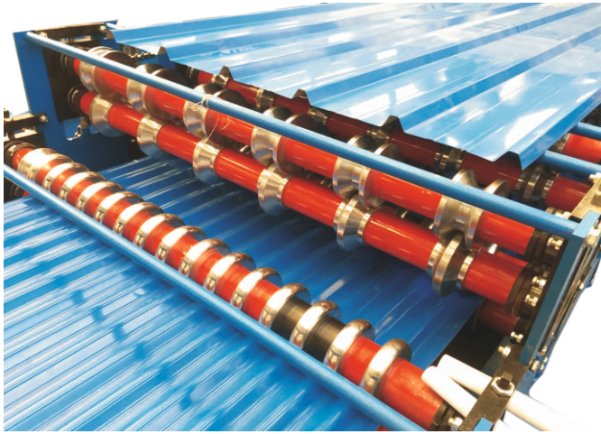
DOUBLE LAYER ROLL FORMING MACHINE
